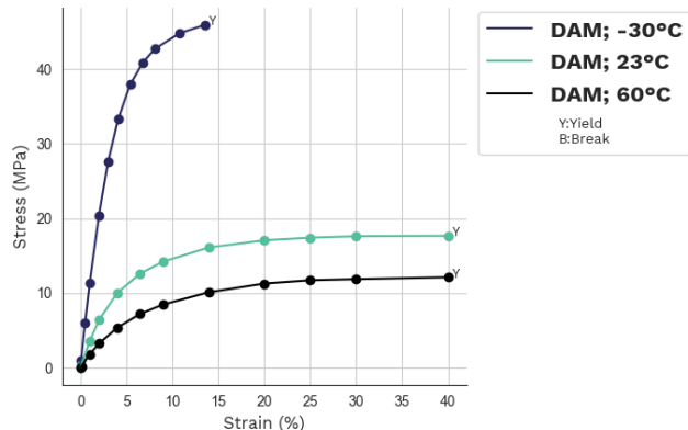
Stress-strain Pebax® 6333 SP 01
