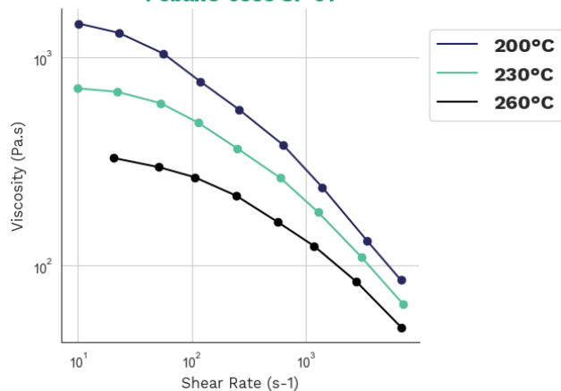
Viscosity-shear rate Pebax® 6333 SP 01
